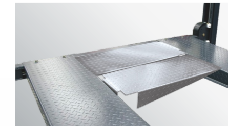
▲ Aluminum alloy drive-in ramps Weight for one set (2 pcs) only 18kg Kits No.:40803
