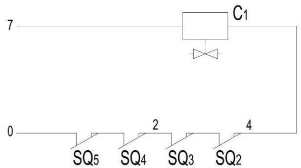
Circuit Diagram Limit Switch (SQ 2 ~SQ 5 ) on Cross Beam
