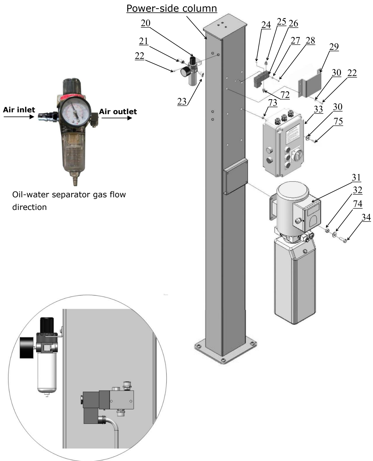
Oil-water separator and Air Solenoid Valve
